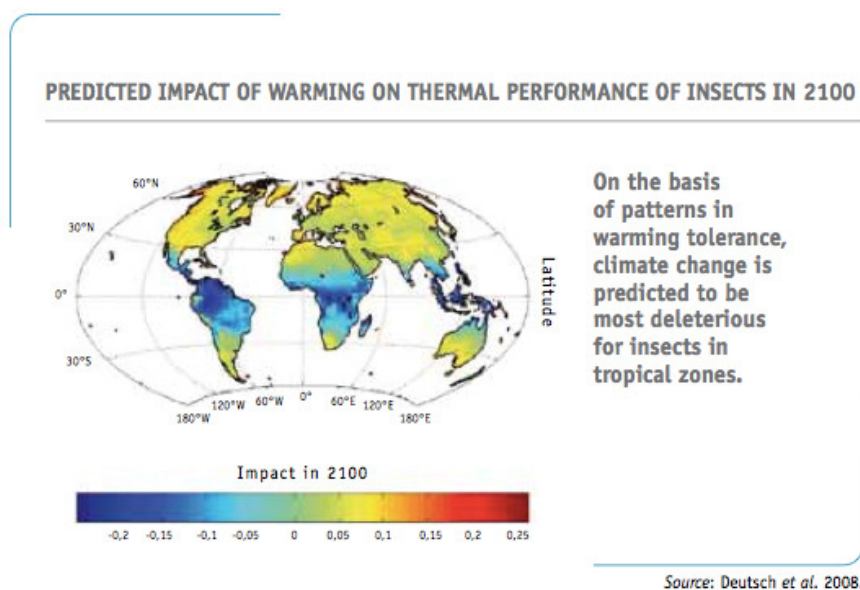
Figure 2. Predicted impacts of warming on insects, 2100 (Deutsch et al 2008)
